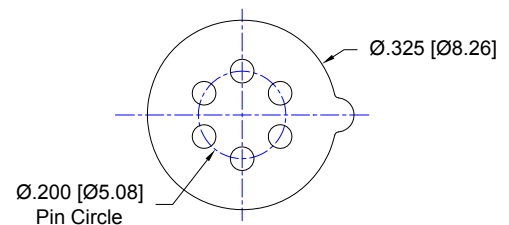
FIG: 2 Thru-Hole: R200-0806-05T- 75S -R27-L14 Surface Mount: R200-0806-05T- 265S -R27-L14
