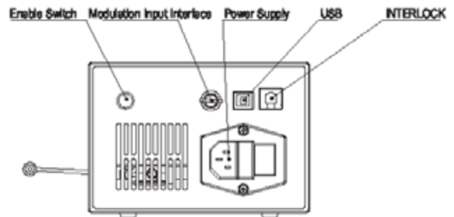
Back View
