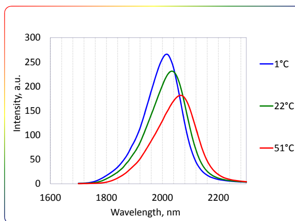
Spectra at different temperatures (qCW, I=150 mA)
