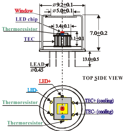
Package TO-5
