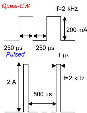
Recommended regimes of LED operation
