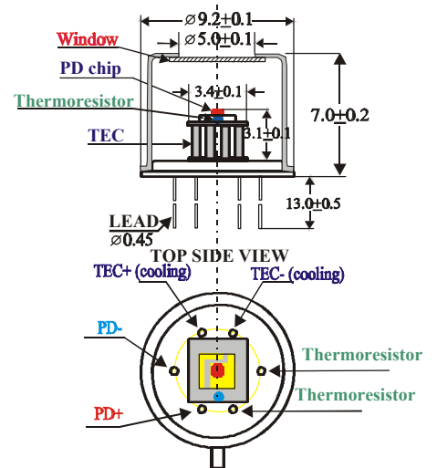
Package TO-5
