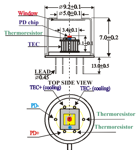
Package TO-5
