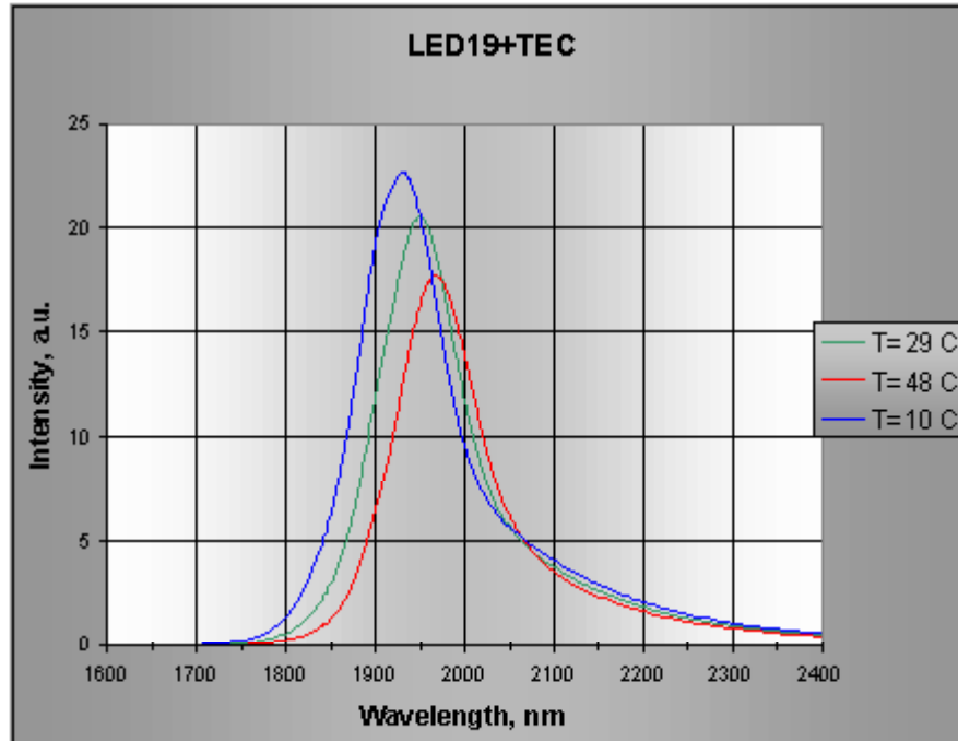
Temperature shift of the LED19 spectra measured in the package with thermocooler
