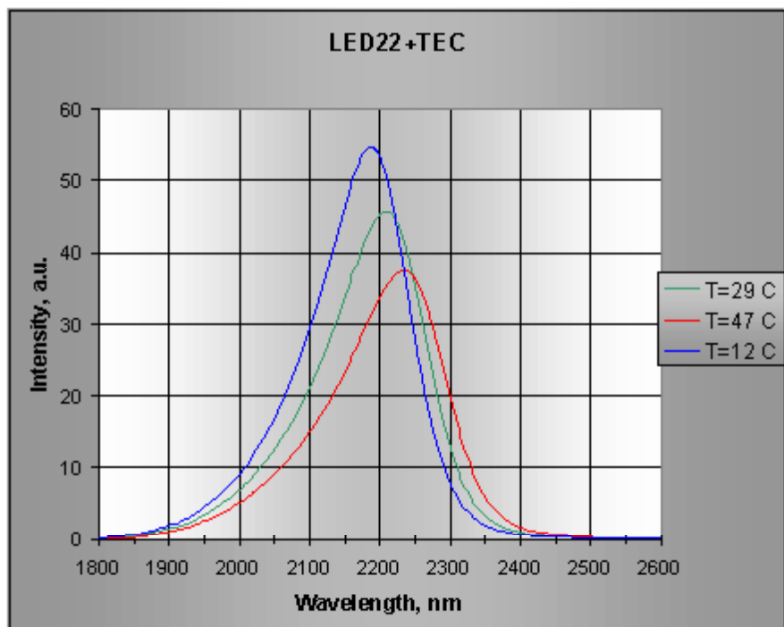
Temperature shift of the LED22 spectra measured in the package with thermocooler
