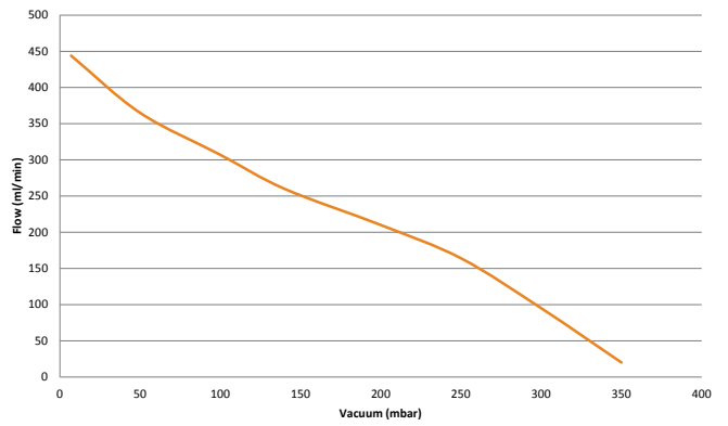
Flow Vs. Vacuum (@ 12V DC)
