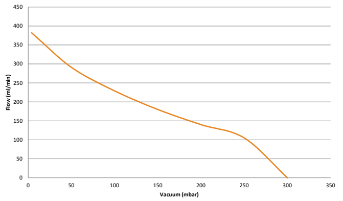
Flow Vs. Vacuum (5V DC)
