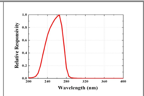
Fig. 2 Responsivity Curve
