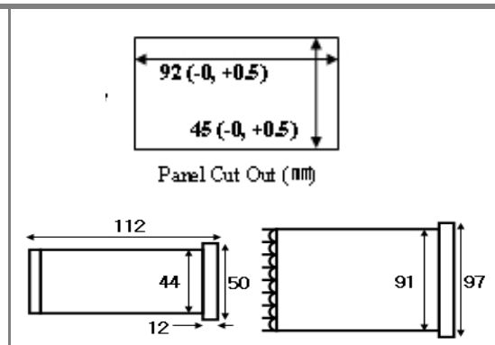
Fig. 2 Size of UV Radiometer 5.0
