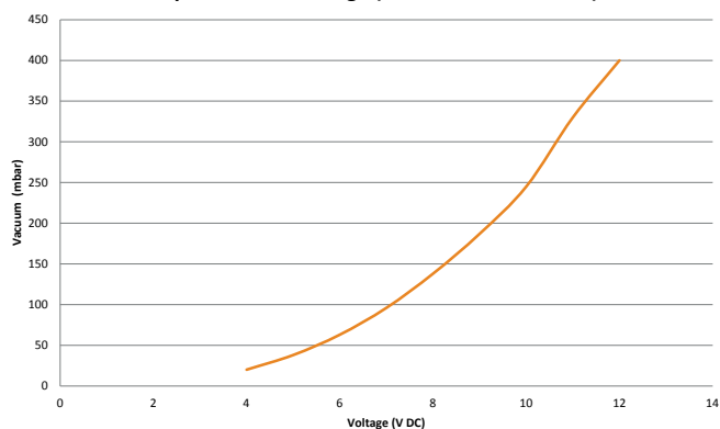
Max pressure Vs. Voltage (@ maximum freeflow)
